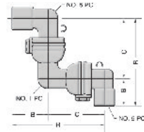
Style No. 70 (Two Planes of Rotation)
